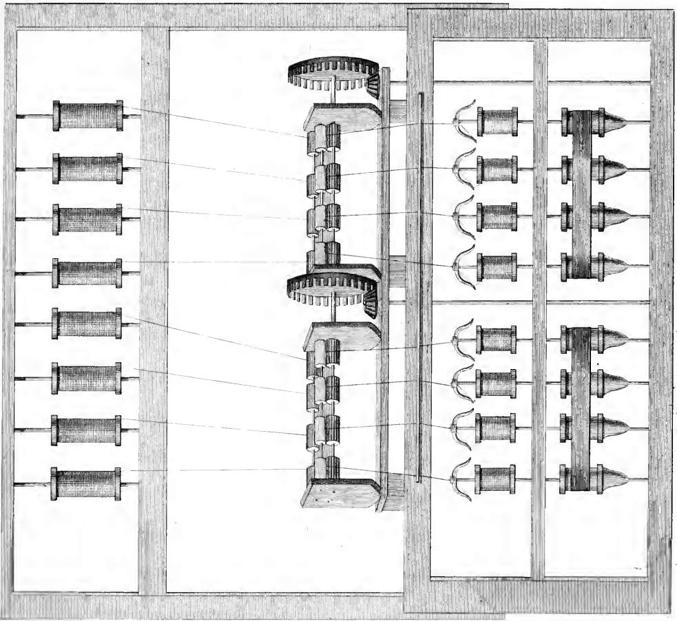
Front view of the Mule Frame.
